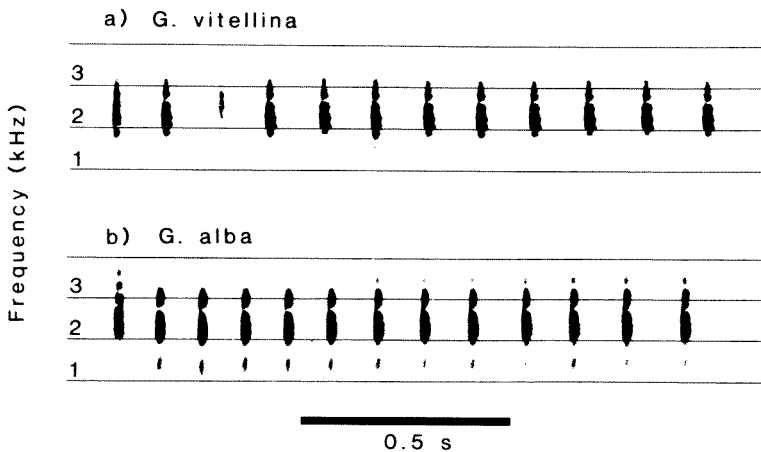
Figure 2 Sound spectrogrammes for a) G. vitellina (soil temperature 14.7°C) b) G. alba (soil temperature 15.4°C.) Both were made with a 45 Hz bandpass filter.
