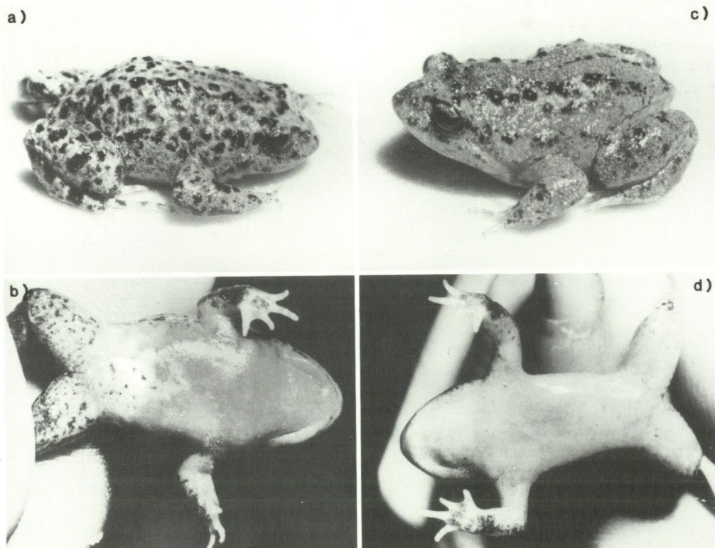
Figure 1 Lectotypes photographed live. a) G. vitellina , lateral view b) G. vitellina ventral view, the darker area extending from the mandibular margin to about half-way between the arms and legs is coloured yellow-orange in life c) G. alba lateral view d) G. alba ventral view, generally white without the yellow-orange area in G. vitellina .
